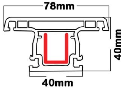
Sliding mullion profile
