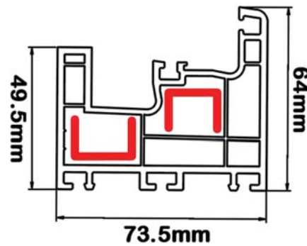
Mono rail frame profile
