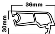
Single glazing bead
