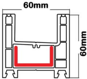
2 track sliding frame profile
