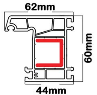
Frame profile
