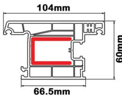
Door sash outward open profile
