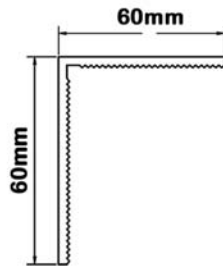
Renovation frame profile
