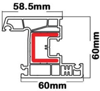
Window Sash profile
