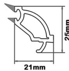
Single glazing bead
