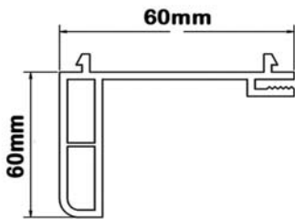
Renovation frame model profile
