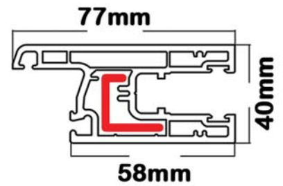
Sliding window sash profile
