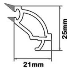
Double glazing bead
