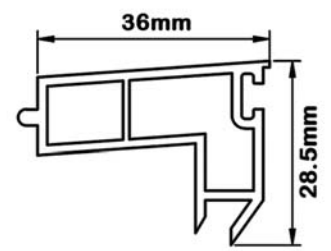
Mono rail cover profile
