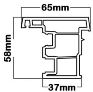
Lap joint profile
