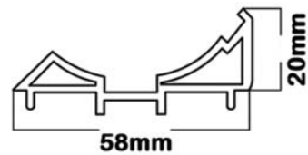
Pipe adaptor profile
